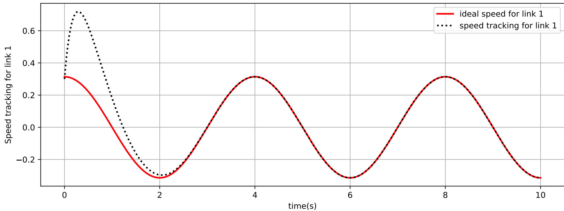
Speed Tracking Performance ( S=2 , S1=1 , m=5 )
